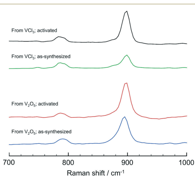
Fig. 4 Raman spectra of [\text{V}(\text{OH})\text{ndc}]_n obtained from \text{V}_2\text{O}_5 and from \text{VCl}_3 before and after activation.
