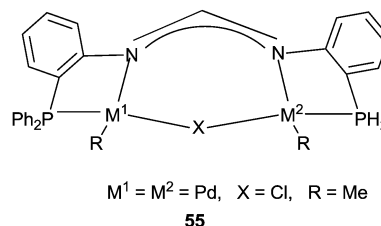
Scheme 67 Reagents and conditions: iodobenzene (5.0 mmol), amine (7.5 mmol), \text{K}_3\text{PO}_4 (5.0 mmol), 1,4-dioxane (3 mL), 55 (0.01 mol%), CO (10 atm), temp. 100 °C, time 15 h.
