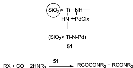
Scheme 63 Reagents and conditions: 51 /PhI (0.5%), phenyl halide (5.1 mmol), \text{E}_2\text{NH} (100 mmol), temp. 100 °C, CO pressure (3.0 MPa), time 6–24 h.
