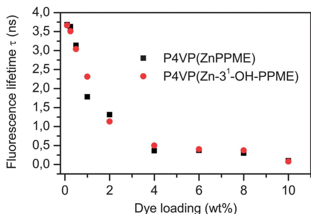
Fig. 7 The fluorescence lifetimes for P4VP(ZnPPME) and P4VP(Zn-3¹-OH-PPME) assemblies given as a function of dye weight percent.
