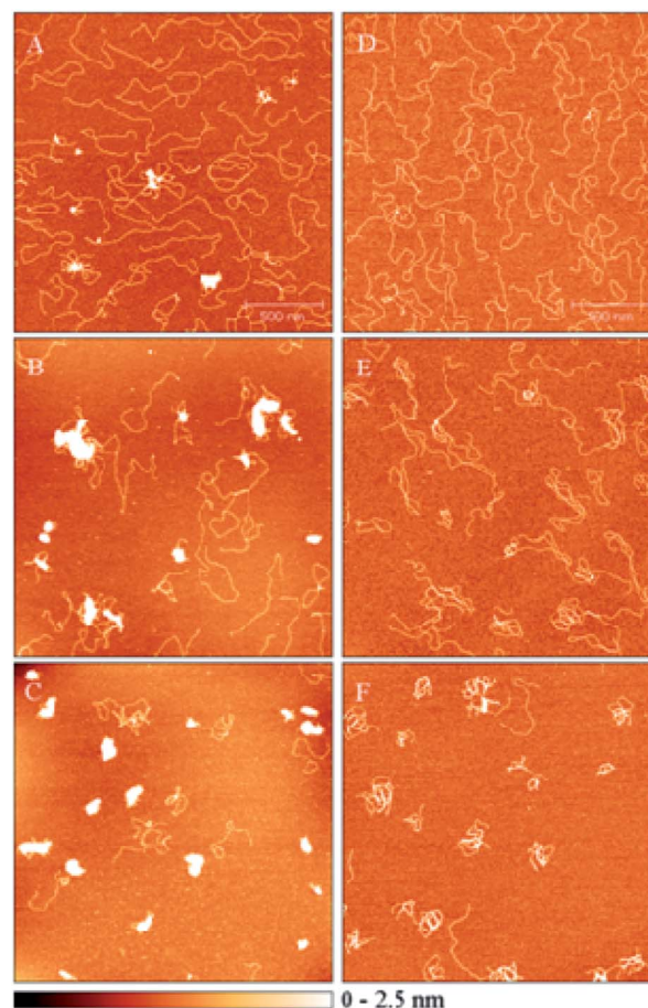
Fig. 3 AFM images of linear plasmid pSP73 (2464 bp) mixed with flexicates at various DNA base : flexicate ratios. (A–C) DNA with Δ-Fe 2 L 1a 3 Cl 4 at 5 : 1, 3 : 1 and 2 : 1 ratios, respectively. (D–F) DNA with Δ-Fe 2 L 2a 3 Cl 4 at 1 : 2, 1 : 4 and 1 : 6 ratios, respectively.
