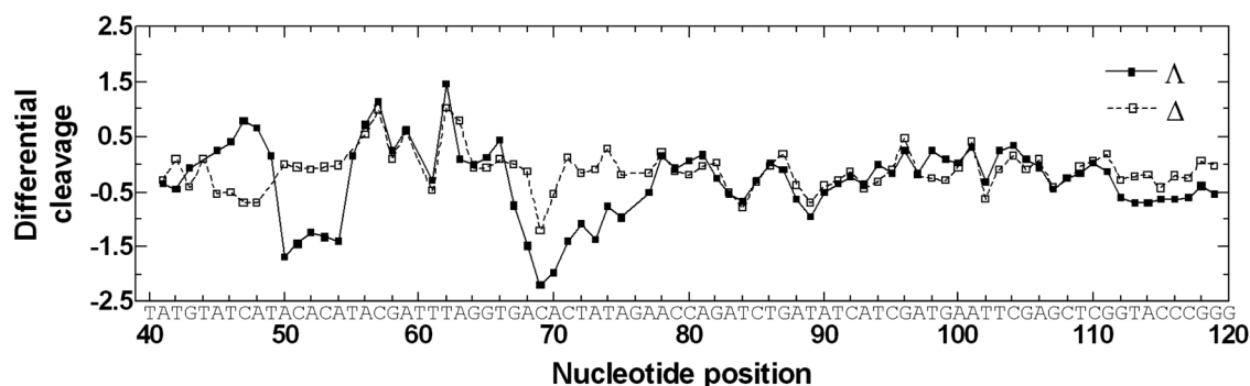
Fig. 7 Caption differential cleavage plots for the \Lambda_{\text{Fe}} - and \Delta_{\text{Fe}} -enantiomers of [\text{Fe}_2\text{L}^{1a}_3]\text{Cl}_4 showing the induced differences in susceptibility to DNase I digestion on the 158 bp HindIII/NdeI restriction fragment of the plasmid pSP73 at 10 : 1 (DNA base : flexicate) ratio. The vertical scale is in units of \ln(f_c) - \ln(f_0) , where f_c is the fractional cleavage at any bond in the presence of flexicate and f_0 is the fractional cleavage of the same bond in the control. Positive values indicate enhancement, negative values indicate inhibition.
