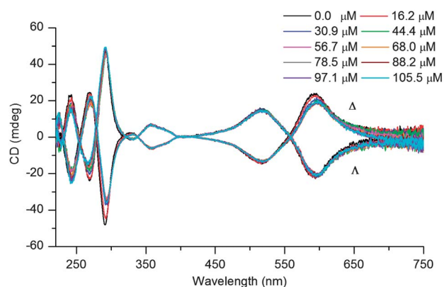
Fig. 4 CD titration series for Δ-Fe 2 L 1a 3 Cl 4 at constant flexicate concentrations (15 μM) and increasing ct-DNA concentrations (indicated in legend). TRIZMA® base buffer (1 mM, pH 7.2). Path length 1.0 cm.
