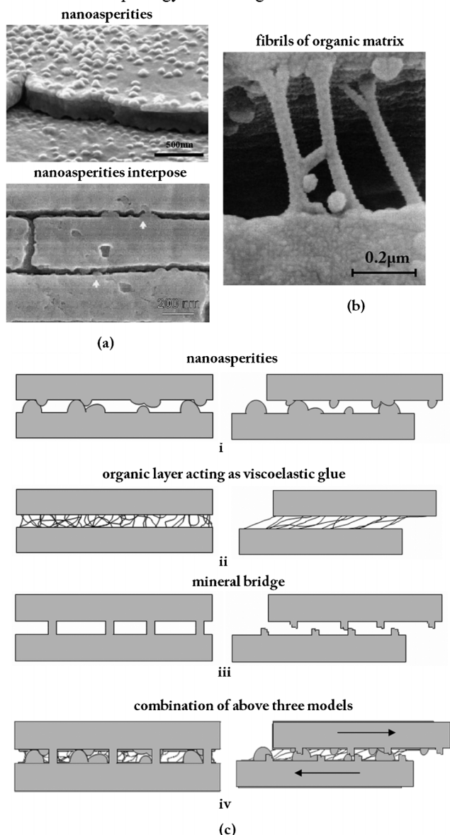
Fig. 12 (a) Asperities (a fraction of which are remnants of mineral bridges); 68 cross section of abalone nacre showing the detailed structure at the lamellae boundaries, where arrows highlight locations where the nanoasperities interpose; 5 (b) fibrils of the organic matrix bridging a delamination crack. Note the large extension and 'splayed-out' anchorage points. 13 (c) Different models for sliding between tiles: 79 (i) inter-tile layer formed by asperities; (ii) organic layer acting as viscoelastic glue; (iii) mineral bridges; (iv) combination of the three mechanisms.
