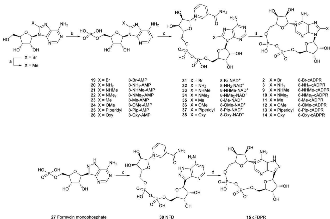
Scheme 1 Synthesis of 8-modified cADPR analogues. Reagents and conditions: (a) PdCl 2 , PPh 3 , AlMe 3 , THF, reflux, 2.5 h. (b) POCl 3 , TEA, 0 °C. (c) ̢-NMN + , DCC, pyridine:water (4 : 1), 7 days, rt. (d) Aplysia cyclase, 25 mM HEPES (pH 6.8), 20 min, rt.
