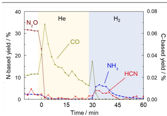
Fig. 8 Yields of gaseous products (HCN (C-based), CO (C-based), \text{N}_2\text{O} (N-based), and \text{NH}_3 (N-based)) determined by FTIR spectroscopy during the reaction \text{CH}_4\text{-NO} (before 0 min), He purging (0–28 min), and \text{H}_2 treatment (after 28 min).
