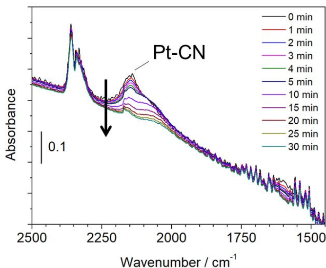
Fig. 7 In situ FTIR spectroscopy results for the reaction of \text{CH}_4 and \text{NO} followed by He purge and hydrogen treatment on the \text{Pt}/\text{Al}_2\text{O}_3 catalyst at 425^\circ\text{C} . Time (min) indicates that treated with hydrogen.
