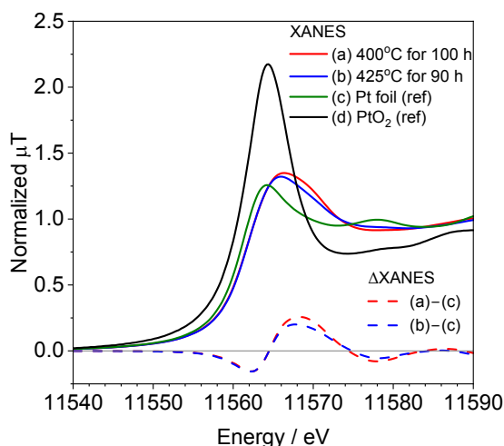
Fig. 3 Pt L_3 -edge XANES spectra of the Pt/ Al_2O_3 catalyst after the reaction with methane and nitric oxide at 400°C for 100 h or 425°C for 90 h, and the difference XANES spectra of the spent catalysts subtracted from the spectrum of Pt foil.
