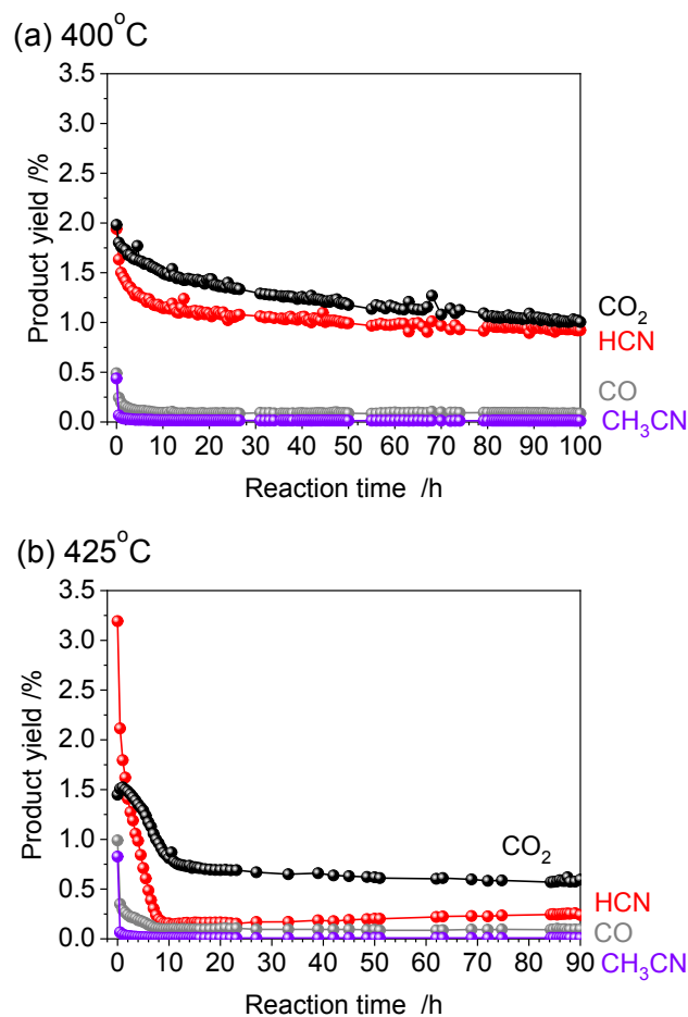
Fig. 2 Time-course of the reaction for methane with nitric oxide over Pt/Al 2 O 3 catalyst at 400°C (a) and 425°C (b). Reaction conditions: 5wt% Pt/Al 2 O 3 (100 mg), CH 4 : NO: He = 13.4: 1.8: 84.8 (total flow rate: 100 mL min -1 ), and 0.1 MPa.
