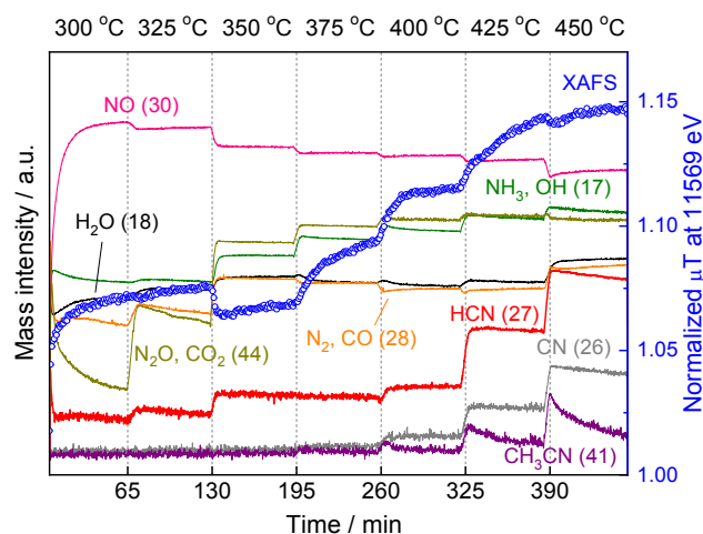
Fig. 4 Changes of MS spectra and the XAFS intensity (at 11569 eV) at various temperatures raising from 300 to 450°C with 25°C steps. Reaction conditions: 5wt% Pt/Al 2 O 3 (100 mg), CH 4 : NO: He = 13.4: 1.8: 84.8 (total flow rate: 100 mL min -1 ), and 0.1 MPa.
