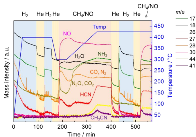
Fig. 5 The time profiles of operating temperature, gas composition, and obtained MS spectra.
