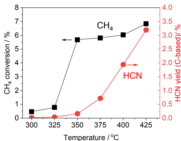
Fig. 1 Methane conversion and hydrogen cyanide yield (carbon-based) as a function of temperature for the reaction of methane with nitric oxide over Pt/Al 2 O 3 catalyst. Reaction conditions: 5wt% Pt/Al 2 O 3 (100 mg), CH 4 : NO = He = 13.4: 1.8: 84.8 (total flow rate: 100 mL min -1 ), and 0.1 MPa.
