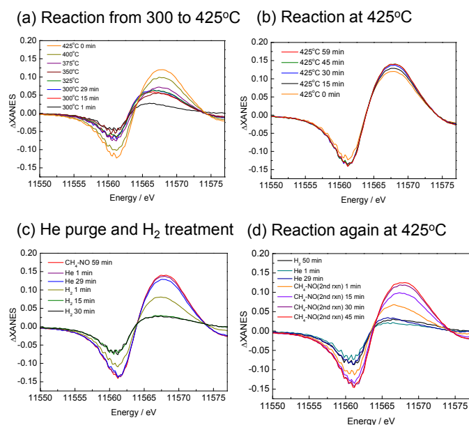
Fig. 6 Pt L_3 -edge XANES difference spectra subtracted from the spectrum just before the introduction of \text{CH}_4 and \text{NO} mixture. (a) reaction from 300 to 425^\circ\text{C} , (b) reaction at 425^\circ\text{C} , (c) He purge and \text{H}_2 treatment after the first reaction at 425^\circ\text{C} , (d) the second reaction at 425^\circ\text{C} after He purge and \text{H}_2 treatment.
