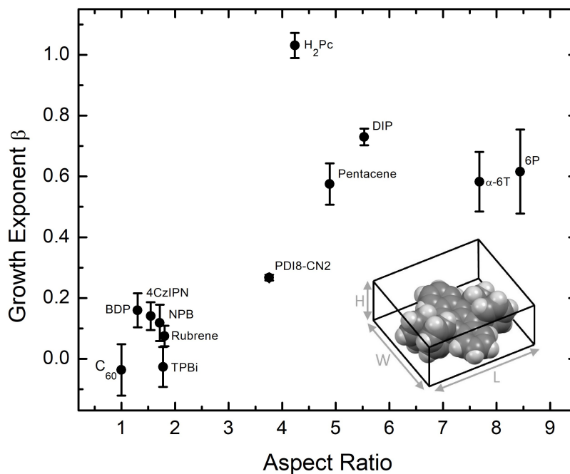
Figure 3: Growth exponent \beta versus molecular aspect ratio. The aspect ratio is defined as the longest dimension divided by the shortest dimension of a box containing a given molecule, as illustrated in the lower-right for rubrene. Errors bars show one standard deviation of the fit data.
