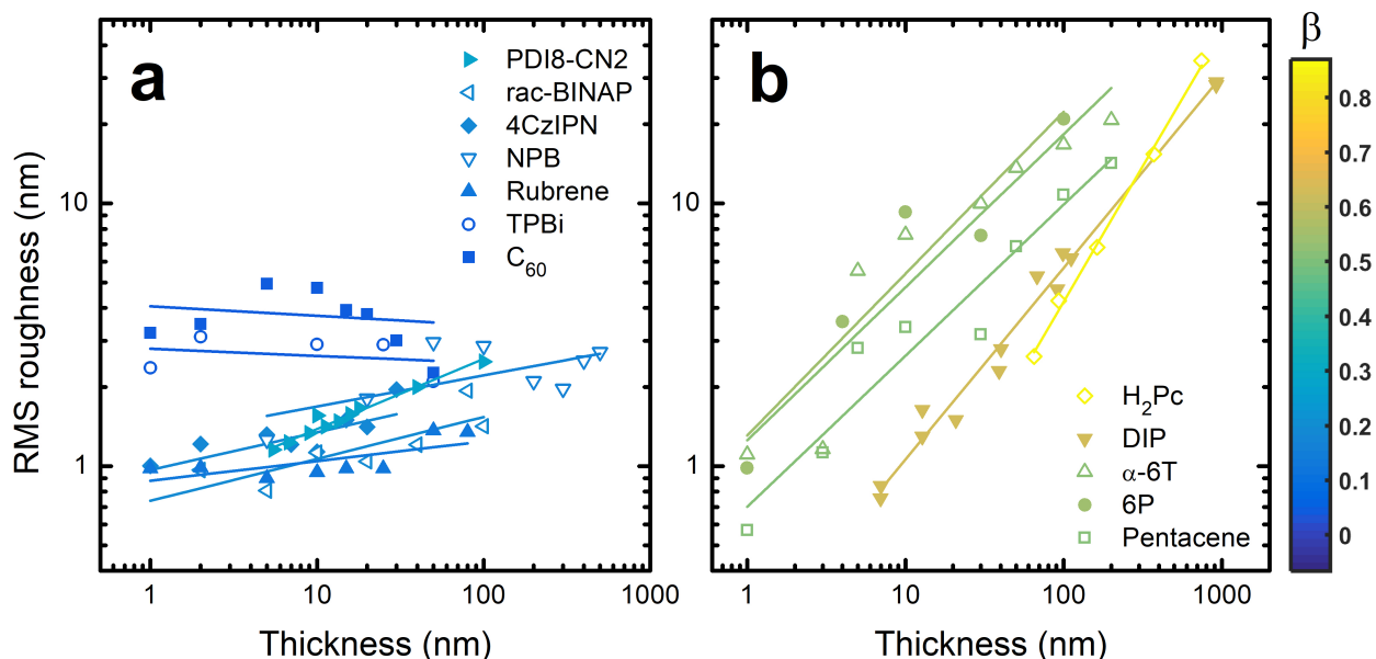
Figure 2: Root mean square roughness versus film thickness for materials considered in this work and from literature. The data are separated for clarity with the materials that remain smooth (lower \beta ) in (a) and materials that become rough (higher \beta ) in (b). The color of each data set corresponds the slope of the fit line, which is equal to the growth exponent, \beta .
