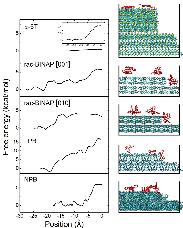
Figure 4: Trajectories of \alpha -6T, rac-BINAP, TPBi and NPB molecules during a step-edge descent and their respective free energy profiles. The molecule's position at the step-edge after descent corresponds to 0 Å. For rac-BINAP the trajectories in both the [010] and [001] directions are shown.
