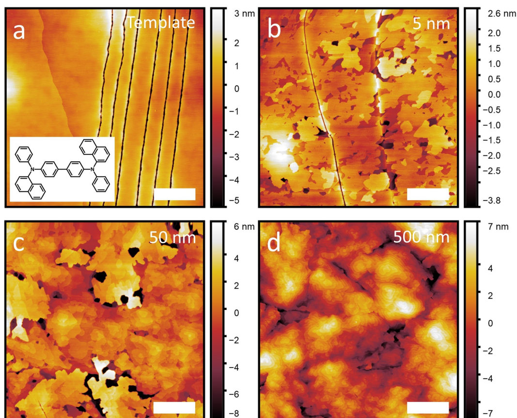
Figure 1: Atomic force microscope images of an (a) NPB template crystal and (b) 5 nm, (c) 50 nm and (d) 500 nm of additional NPB grown on top of the template. Scale bars are 1 \mu\text{m} . Molecular structure of NPB is shown as an inset in (a).
