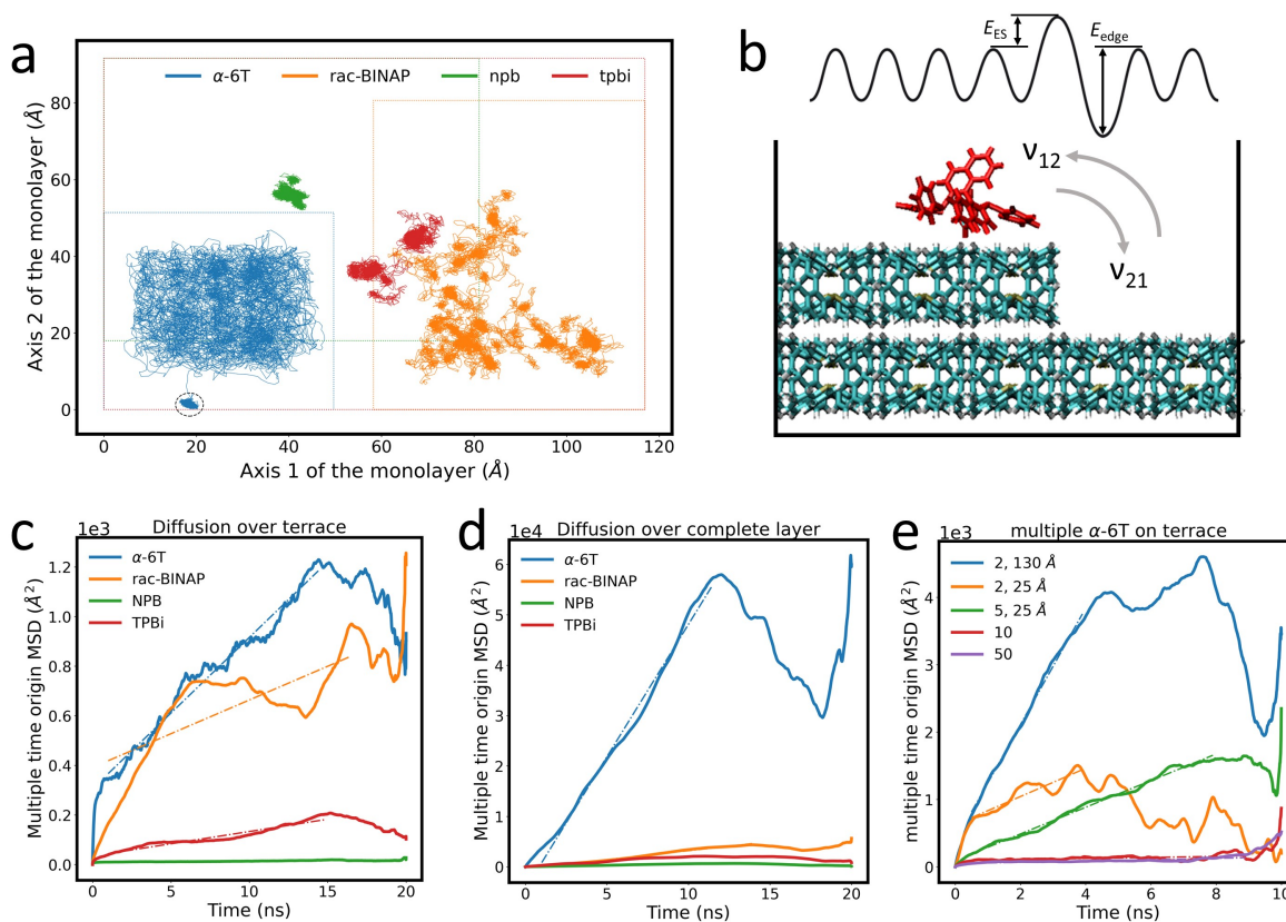
Figure 5: (a) Trace of the center of mass of ad-molecules traversing a molecular terrace. The dashed circle indicates the \alpha -6T ad-molecule spontaneous descent over the island layer edge after 14 ns. The boundary of each terrace is marked as a dashed line of the same color as the molecular trajectory. Traces are shifted for clarity. (b) Illustration of the rates of ascent and descent as well as E_{ES} and E_{edge} in a simplified representation of a complex 3D molecular surface. Calculations of MSD for (c) diffusion over a terrace and (d) diffusion over a complete monolayer. (e) Calculations of MSD of 2, 5, 10 and 50 \alpha -6T ad-molecules on an \alpha -6T surface. The distance value in the legend indicates the initial center of mass distance between each ad-molecule. The initial distance is 5 Å if no specification is given. The 2 ad-molecules system with 130 Å initial distance formed an aggregate after 4 ns and 2 ad-molecules with 25 Å initial distance formed an aggregate shortly after the simulation started (i.e. within 0.5 ns). Dashed lines in (c), (d), and (e) are fits to the MSD data to determine the diffusion coefficient and are listed in the SI.
