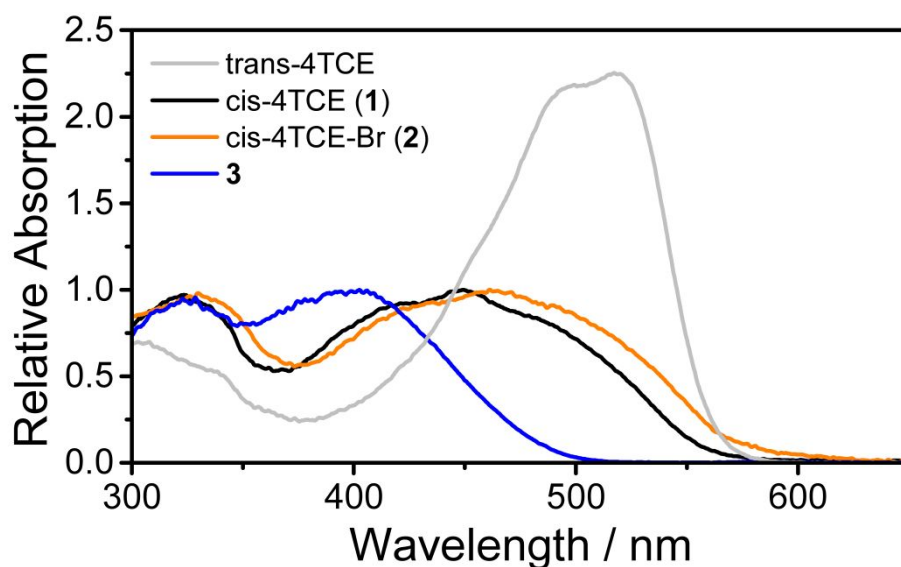
Figure 1: Steady-state UV/Vis absorption spectra for trans-4TCE (grey), cis-4TCE (( 1 ) black), cis-4TCE-Br (( 2 ) orange) and the bis(bithienyl) perfluorocyclopentene (( 3 ) – blue). Spectra for 1-3 are normalized to peak intensity; trans- and cis-4TCE are presented at relative absorptivities.
