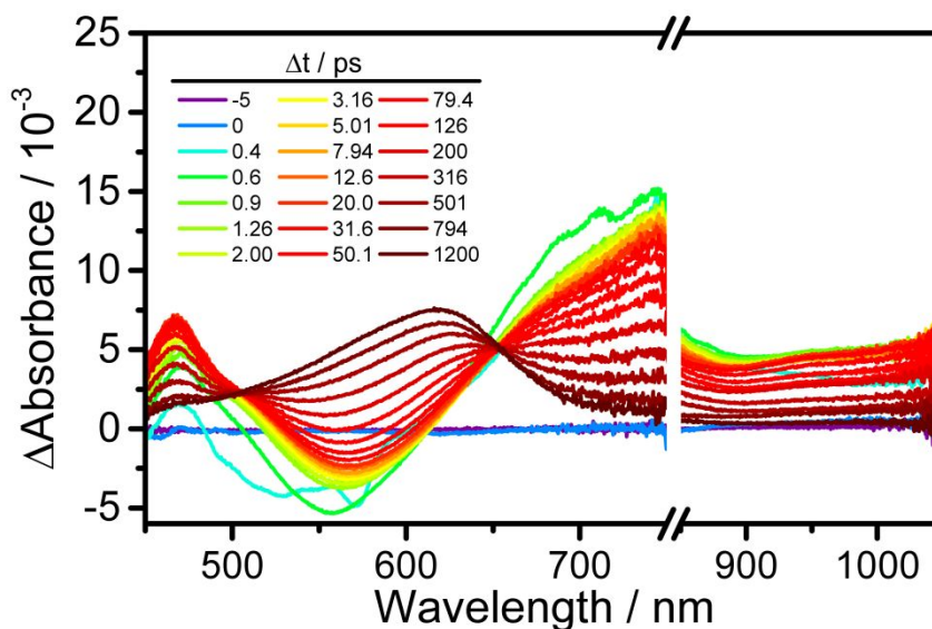
Figure 7. Transient spectra for 3 collected with 490 nm excitation.
