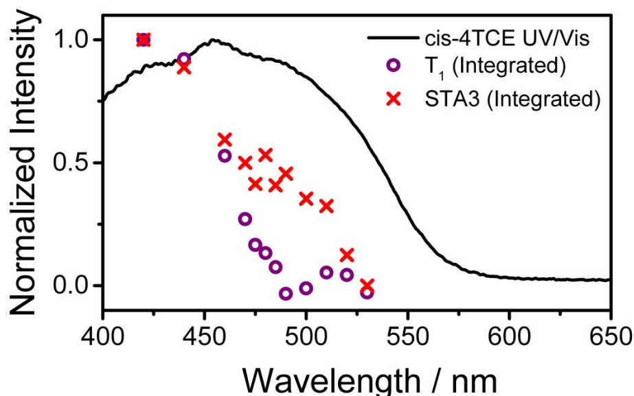
Figure 6: Relative intensities of TA spectral features (integrated 525-575 nm for STA3, 600-700 nm for T 1 absorption) observed for 4TCE with excitation wavelength compared to the cis-4TCE absorption spectrum. Traces/spectra are normalized to their peak intensities.
