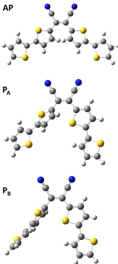
Figure 9: Molecular geometries calculated at the M052X level of theory utilizing a 6-31g* basis set. The two parallel structures, P A and P B , are energetically separated by only 33.8 cm -1 . The ‘anti-parallel’ (AP) conformer lies approximately 450 cm -1 higher than P A .
