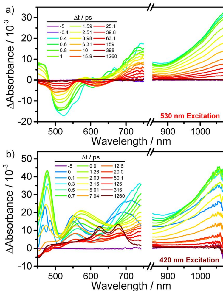
Figure 2: Transient absorption spectra of cis-4TCE ( 1 ) (at representative time delays, \Delta t ) collected with (a) low energy (530 nm) and (b) high energy (420 nm) excitation.
