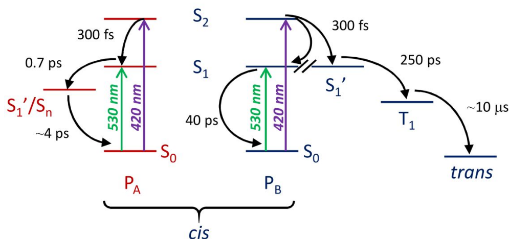
Figure 10. Jablonski diagram of energy- and conformer-dependent photophysics of cis-4TCE
