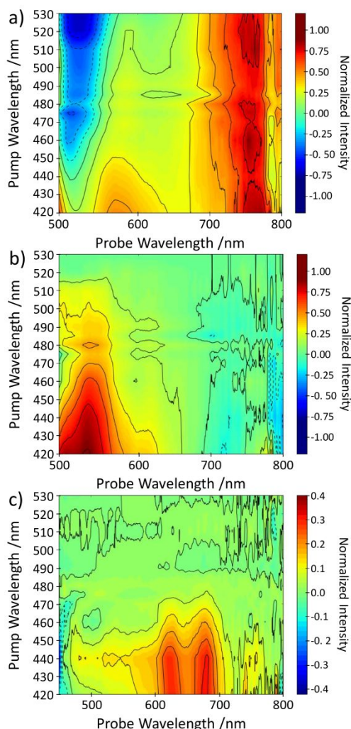
Figure 5: Excitation wavelength-dependence of 4TCE TA spectral features. a) Excitation wavelength-dependence of TA spectra collected with a 1 ps pump-probe delay (normalized at ~750 nm). b) Wavelength dependent difference spectra at 1 ps delay obtained by subtracting the normalized TA spectrum collected at 530 nm to highlight excitation dependence of the 530 nm absorption feature (“STA3”). c) Wavelength dependent spectra collected 500 ps following excitation to highlight onset for the appearance of T_1 absorption.
