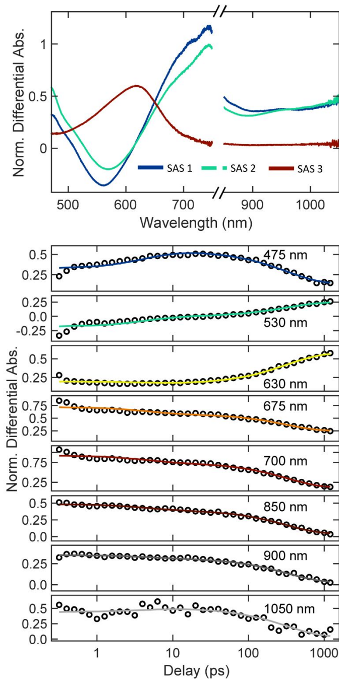
Figure 8. Global fitting results for TAS data collected with 490-nm excitation of 3 . (a) Species-associated spectra (SAS) for a three-component sequential kinetic model. (b) Time-dependent fits to transients at representative probe wavelengths. Data was normalized to intensity at 725 nm at 1 ps before global fitting.
