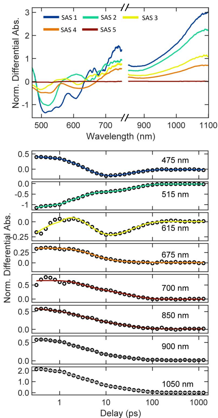
Figure 3: Global fitting results for TAS data collected with 530-nm excitation of cis-4TCE. (Top) Species-associated spectra (SAS) for five-component sequential kinetic model. (Bottom) Time-dependent fits to transients at representative probe wavelengths. TAS data was normalized at 750 nm prior to global analysis to facilitate comparisons between SAS and temporal cuts for different excitation wavelengths.
