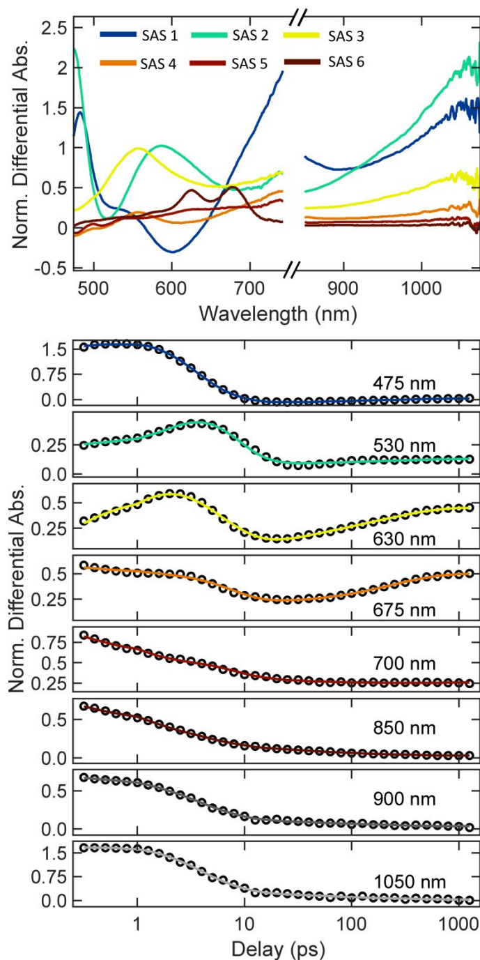
Figure 4: Global fitting results for TAS data collected with 420-nm excitation of cis -4TCE. (Top) Species-associated spectra (SAS) for six-component sequential kinetic model. (Bottom) Time-dependent fits to transients at representative probe wavelengths. TAS data was normalized at 740 nm prior to global analysis to facilitate comparisons between SAS and temporal cuts for different excitation wavelengths.
