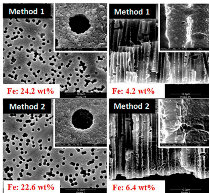
Figure 7. Visualization by SEM and quantification by EDX of MNP loading for hydrogel pore-filled membranes obtained by the two different methods.
