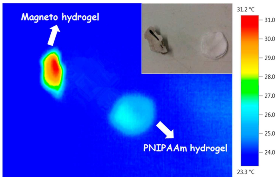
Figure 5. Thermal images of magneto-hydrogel and reference material without MNP after 1 minute of AMF exposure ( I = 15.6 A, f = 745 kHz, H \sim 20 kAm -1 ).
