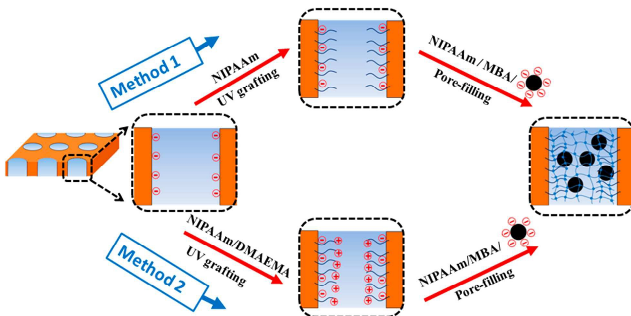
Figure 2. Schematic illustration of methods to fabricate magneto-responsive membranes: as first step surface-grafting of linear polymer chains as anchor for the hydrogel network prepared in second step via in situ cross-linking polymerization.
