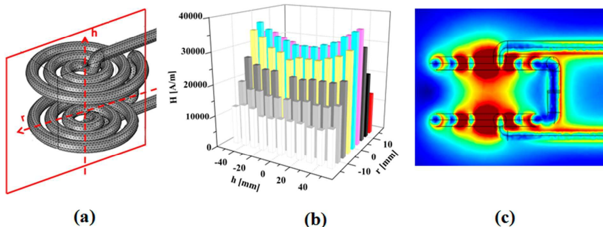
Figure 3. Electro-magnetic field amplitude distribution between the two inductor coils; (a) geometry of the inductor coils and placing of coordinates; (b) measured field amplitude distribution with current input of 15.6 A and frequency of 745 kHz; (c) computer simulation of field amplitude distribution (highest intensities red, lowest blue; no scale used because simulation had been done with other current and frequency input parameters than in experiments).
