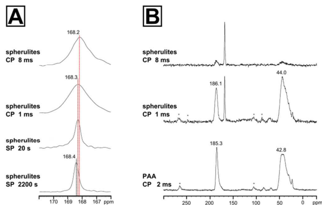
Fig 2 13 C solid state NMR spectra of the calcite spherulites evidencing the presence of a second amorphous phase and the incorporation of the polymeric additive PAA into the spherulites at grain boundaries. A Carbonyl region of the 13 C solid state NMR spectra of the calcite spherulites, recorded as single pulse (SP) experiments with 2200 s or 20 s recycle delay, and 1 H- 13 C cross-polarization transfer (CP), recorded with 3 s recycle delay at 1 ms and 8 ms contact time. B 13 C CP NMR spectra of the spherulites and of the pure PAA polymer standard recorded with 2 ms cross-polarization time. The signal at 185.3 ppm with a full width at half height (FWHH) of 457 Hz of the PAA spectrum corresponds to the 13 C resonance of the carbonyl group, the broad signal at 42.8 ppm with a FWHH of 1578 Hz is related with the overlapping CH and CH 2 signals of the vinyl backbone of the polymer. Additionally, two broad spinning sidebands, spaced by the spinning frequency, are observed at ca. 105 and 265 ppm which arise from the significant chemical shift anisotropy of the carbonyl group.
