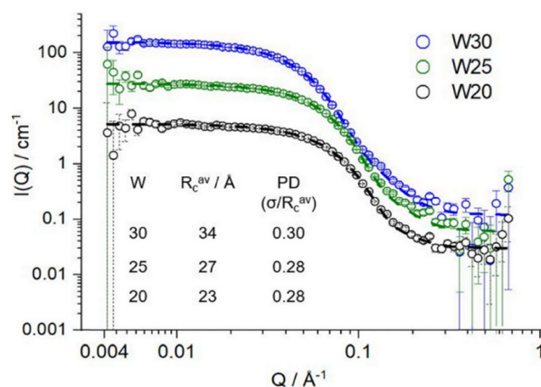
Fig. 6 Core-contrast SANS profiles (D 2 O/H-surf//H-oil: D/H/H) for AOT-SiB W/O- \mu Es in toluene, [surf] = 0.050 M, temperature: 298 K; data and fits to the polydisperse P(Q) model (dashed lines) were multiplied by (blue) × 6 and (green) × 3 for better visualization.
