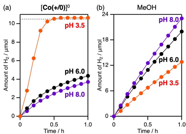
Fig. 5 Time courses of H 2 evolution using CrO x /Pt/SrTiO 3 :Rh (10 mg) in an aqueous solution (70 mL) containing (a) 0.3 mM [Co(+/0)] 0 or (b) 10 vol% MeOH as an electron donor at pH 3.5, 6.0, or 8.0 (adjusted with HCl) under visible-light irradiation ( \lambda = 430 nm).
