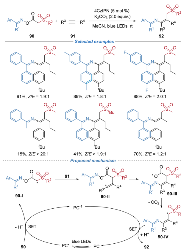
Scheme 33 Oxime esters as bifunctional reagents for radical alkylamination of alkynes.
