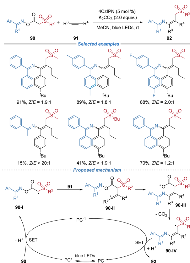
Scheme 33 Oxime esters as bifunctional reagents for radical alkylation of alkynes.
