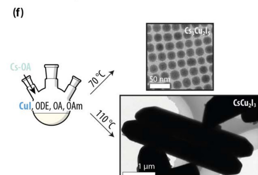
Fig. 12 Caesium copper halides as representative of copper halide SNCs. (a) Unit cell, copper cluster geometry, and simulated XRPD patterns of the most common compositions reported for Cs–Cu–X (where X = Cl, Br, I). (b) Absorption (dashed lines) and emission (solid lines) spectra of \text{Cs}_3\text{Cu}_2\text{I}_5 (blue) and \text{CsCu}_2\text{I}_3 (yellow), alongside a photo of the dispersion under UV excitation, and the corresponding photoluminescence decay curves. Adapted with permission from ref. 286, Copyright 2019, American Chemical Society. (c) The emission stems from a self-trapped exciton. (d) Representation of the Jahn–Teller distortion that occurs after excitation in \text{Cs}_3\text{Cu}_2\text{I}_5 . Adapted with permission from ref. 287, Copyright 2025, Springer. (e) Absorption and emission spectra, photoluminescence decay curves, and photo under UV excitation of a series of alloyed \text{Cs}_3\text{Cu}_2\text{X}_5 SNCs, alongside \text{Cs}_3\text{Cu}_2\text{Cl}_3 SNCs. Adapted with permission from ref. 288, Copyright 2020, American Chemical Society. (f) Scheme of the synthesis protocol for the synthesis of \text{Cs}_3\text{Cu}_2\text{I}_5 SNCs or \text{CsCu}_2\text{I}_3 microcrystals, alongside the TEM images of the respective materials. Adapted with permission from ref. 284, Copyright 2019, John Wiley and Sons. (g) TEM images of \text{Cs}_3\text{Cu}_2\text{I}_5 SNCs obtained using different halide additives, showing optimized morphology and narrow size distribution in the presence of \text{MnI}_2 . Adapted with permission from ref. 289, Copyright 2022, American Chemical Society. (h) TEM images of parent \text{Cs}_3\text{Cu}_2\text{Cl}_5 synthesized at 180 °C and used as sacrificial species for cation exchange with Zn, Bi, and Cd. The TEM images of the SNCs obtained from the cation exchange procedures are reported in the bottom row. Adapted with permission from ref. 290, Copyright 2023, American Chemical Society.
