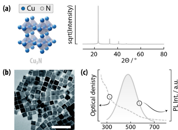
Fig. 4 Copper nitride SNCs. (a) Unit cell and simulated XRPD pattern of \text{Cu}_3\text{N} . (b) TEM image of \text{Cu}_3\text{N} SNCs showing the characteristic cubic morphology. Scale bar is 100 nm. (c) Extinction and emission spectrum of \text{Cu}_3\text{N} SNCs. Adapted with permission from ref. 44, Copyright 2020, Royal Society of Chemistry.
