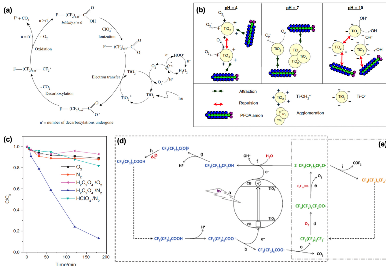
Fig. 5 (a) Proposed photocatalytic decomposition cycle of PFCAs on \text{TiO}_2 under UV light, involving ionization, electron transfer, decarboxylation, and oxidation. Successive \text{CF}_2 -unit losses yield shorter-chain PFCAs until complete mineralization to \text{CO}_2 and \text{F}^- ions. Reproduced from ref. 186 with permission from Elsevier BV, copyright 2009; (b) schematic of \text{TiO}_2 surface charge effects on PFOA degradation across pH: \text{Ti}-\text{OH}_2^+ dominates at acidic pH, \text{Ti}-\text{OH} at neutral (pH 6–7, zero-point charge), and \text{Ti}-\text{O}^- at basic pH. Despite expected higher degradation at low pH due to electrostatic attraction, experiments showed greater PFOA removal at basic pH (10), indicating that radical-driven processes outweigh surface charge effects. Reproduced from ref. 187 with permission from Elsevier BV, copyright 2009; 187 (c) photocatalytic degradation of PFOA by \text{TiO}_2 under 254 nm UV. Adsorption was <8%. After 180 min, removal reached 10.5% ( \text{O}_2 ), 12.4% ( \text{N}_2 ), 6.6% with oxalic acid ( \text{O}_2 ), and 86.7% with oxalic acid ( \text{N}_2 ). At pH 2.47 ( \text{HClO}_4 ), only 17.8% removal occurred. Rate constants were 1.16 \times 10^{-2} \text{ min}^{-1} (oxalic acid) vs. 1.0 \times 10^{-3} \text{ min}^{-1} ( \text{HClO}_4 ). Defluorination was 16.5% with \text{TiO}_2 /oxalic acid but <1% otherwise. Reproduced from ref. 188 with permission from Elsevier BV, copyright 2011; proposed reaction mechanism for PFOA degradation in the presence of a \text{TiO}_2 photocatalyst, incorporating both photo-redox (d) and \beta -scission (e) pathways. Reproduced from ref. 189 with permission from Elsevier BV, copyright 2015. 189
