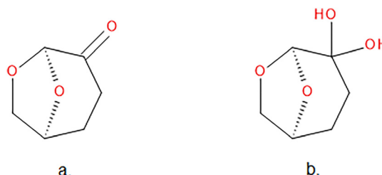
Fig. 4 Structures of Cyrene (a) and Gemdiol (b). In aqueous solution, the carbonyl group of Cyrene undergoes water addition to form the corresponding geminal diol. Equilibrium is established rapidly, with the ratio between the two forms depending on the amount of water present. 20,21
