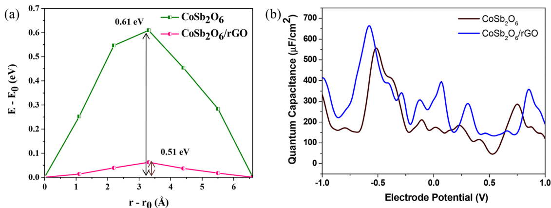
Fig. 9 (a) Diffusion energy plot for the (110) surface of CoSb 2 O 6 and CoSb 2 O 6 /rGO composite systems and (b) plot of the variation of quantum capacitance with electrode potential for the (110) surface of CoSb 2 O 6 and CoSb 2 O 6 /rGO composite systems.
