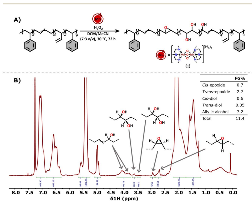
Fig. 4 (A) Catalytic oxyfunctionalisation conditions tested on SBS using the tri-oxo (1) bridged analogue of MnTACN. (B) ^1H NMR spectrum after the oxyfunctionalisation of styrene–butadiene–styrene (SBS) block-co-polymer, with the corresponding FG% of each installed oxyfunctional group.
