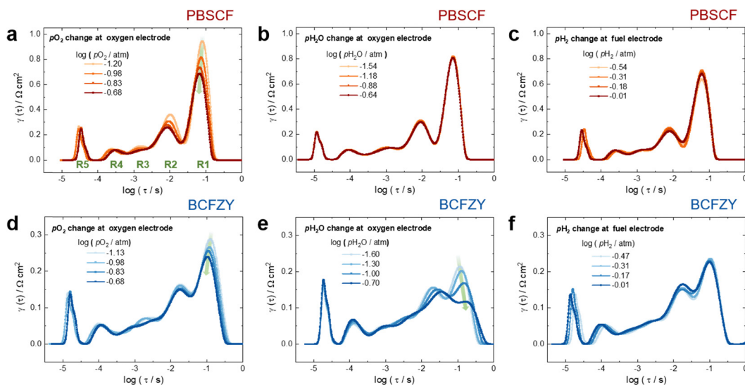
Fig. 6 Distribution of relaxation time (DRT) spectra of PCFCs with PBSCF (top row) and BCFZY (bottom row) cathodes measured at 550^\circ\text{C} under various gas conditions. (a and d) Effect of varying p\text{O}_2 at the cathode, (b and e) effect of p\text{H}_2\text{O} at the cathode (with a constant flow of 3% humidified \text{H}_2 at the anode), and (c and f) effect of p\text{H}_2 at the anode (with a constant flow of dry air at the cathode). Five distinct relaxation processes (R1–R5) are identified, indicating that the total polarization resistance consists of multiple elementary reaction steps.
