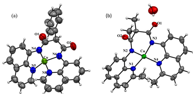
Fig. 1 (a) ORTEP plot of (a) CuL2 (CCDC No. 2491828) and (b) CuL3 (CCDC No. 2477383) shown at the 50% probability level with only heteroatoms bonded. Selective interatomic bond distances and angles for CuL2 : Cu(1)–N(4) = 1.941 Å, Cu(1)–N(5) = 2.015 Å, Cu(1)–N(6) = 1.941 Å, Cu(1)–N(8) = 1.989 Å, [N(4)–Cu(1)–N(5)] = 83.0°, [N(4)–Cu(1)–N(6)] = 98.7°, [N(4)–Cu(1)–N(8)] = 172.9°, [N(5)–Cu(1)–N(6)] = 159.3°, [N(5)–Cu(1)–N(8)] = 97.7°, [N(6)–Cu(1)–N(8)] = 83.2°. CuL3 : Cu(1)–N(1) = 1.997 Å, Cu(1)–N(2) = 1.912 Å, Cu(1)–N(6) = 2.003 Å, Cu(1)–N(8) = 1.914 Å, [N(1)–Cu(1)–N(2)] = 83.6°, [N(1)–Cu(1)–N(4)] = 105.9°, [N(1)–Cu(1)–N(3)] = 156.4°, [N(2)–Cu(1)–N(4)] = 148.0°, [N(2)–Cu(1)–N(3)] = 98.4°, [N(4)–Cu(1)–N(3)] = 84.9°.
