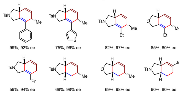
Scheme 31 Co(I)-catalyzed intramolecular [4+2] cycloaddition reactions of unactivated diene-yne and trienes.
