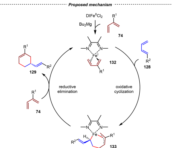
Scheme 29 Fe(I)/ \alpha -diimine-catalyzed asymmetric cross-[4+2] cycloadditions of unactivated 1,3-dienes.
