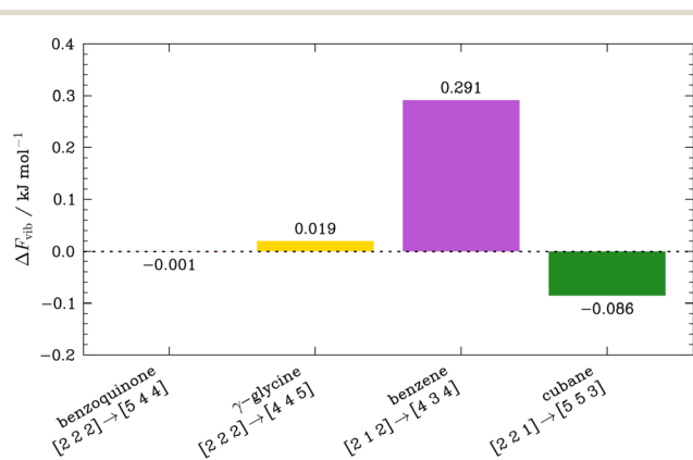
Fig. 6 Change in the vibrational free energy for OMCs as q -point sampling in the Brillouin zone is increased from the coarsest MP grid yielding a stable dispersion (ca. 0.14 \text{ \AA}^{-1} q -point spacing) and the finest MP grid used in this study (ca. 0.04 \text{ \AA}^{-1} q -point spacing), limited by computational cost.
