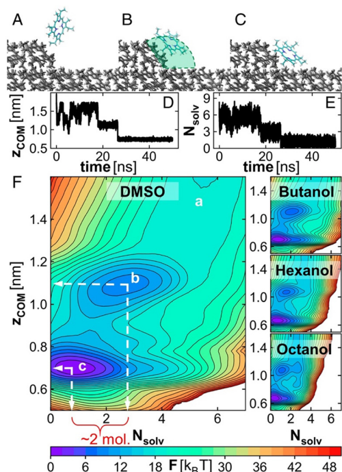
Fig. 13 Microscopic view of the ingress of an etioporphyrin I molecule into a kink. (A–C) Representative snapshots of an etioporphyrin I molecule in the solution near a kink (A), at the intermediate state (B) and at its final location in the kink (C). Classical MD simulation results. The green sphere in (B) defines our choice of the kink cavity, i.e. , the volume where the dynamics of the solute molecule that partake in the reaction between a solute molecule and a kink are evaluated. Solvent molecules are omitted for clarity. The kink is viewed along the unfinished molecular row at the step edge. The direction of step growth is from left to right. Etioporphyrin I molecules in the crystal lattice are shown in gray. The lattice planes of etioporphyrin I molecules in front and behind the plane, which hosts the kink, are omitted. In the incoming etioporphyrin I molecule, C atoms are shown in teal, N in blue and H in silver. (D and E) A representative MD simulation trajectory of an incoming etioporphyrin I molecule displayed in terms of the normal distance z_{\text{COM}} from the center of mass of an incoming molecule to that of the molecule at the bottom surface of a kink in (D) and the number of solvent molecules N_{\text{solv}} in the kink cavity [shown in green in (B)] in (E). (F) Two-dimensional potential of mean force profiles F(N_{\text{solv}}, z_{\text{COM}}) for incorporation of a solute molecule into a kink from the four solvents. F was computed from well-tempered metadynamics simulations. The locations of the three states shown in (A–C) are indicated in the DMSO plot. Reprinted with permission from R. Chakrabarti, L. Verma, V. G. Hadjiev, J. C. Palmer and P. G. Vekilov, Proc. Natl. Acad. Sci. U. S. A. , 2024, 121 , e2320201121. 45
