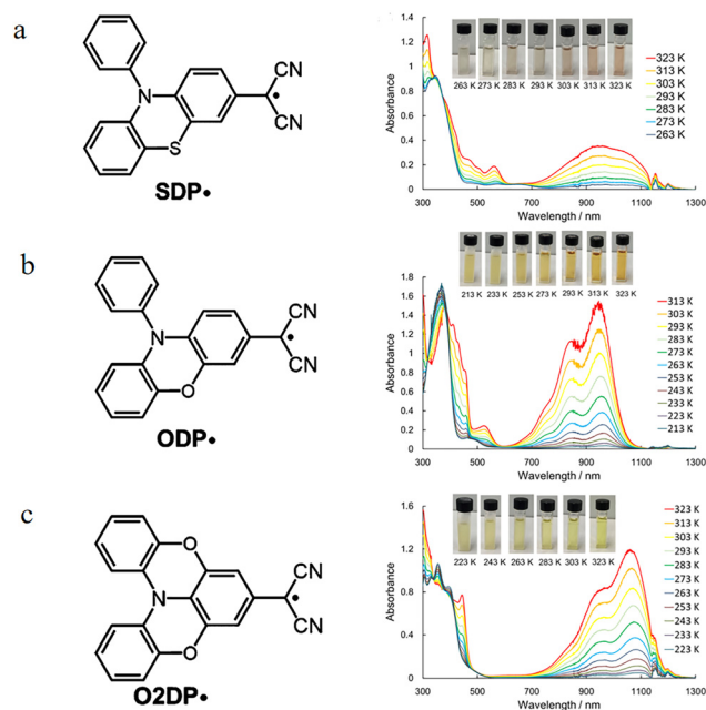
Fig. 15 Molecular structure and corresponding ultraviolet absorption spectra of (a) SDP• and (b) ODP• and (c) O2DP•, reproduced from ref. 49 with permission from American Chemical Society, ACS Materials Letters , 2019, 1, 25–29, copyright 2019.
