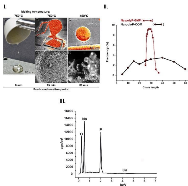
Fig. 1. Synthesis of Na-polyP from NaH 2 PO 4 monomers. The polymer was prepared at 750°C using a controlled polycondensation process, followed by accelerated cooling (B to C). (I) (A) Pouring the melt from the crucible (83 mm upper diameter and 55 mm height). Two time points were chosen to demonstrate polyP lens formation; after a post-condensation period of (D) 15 min and (E) 30 min. Perfectly convex lenses are formed after 30 min. At time point 15 min, the lenses are still fused together. The images (B) and (C) were taken with an infrared camera; the square in (C) is the camera focus. (II) The sharp distribution of polyP chain lengths (given in P i units) of the Na-
