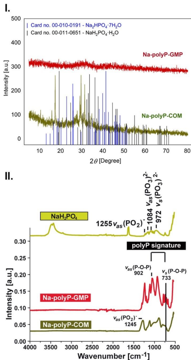
Fig. 3. (I) XRD analyses of Na-polyP-GMP compared to Na-polyP-COM. The commercial product shows some crystalline signals. (II) FTIR analysis. In comparison to the NaH 2 PO 4 starting material, the two Na-polyP preparations Na-polyP-GMP and Na-polyP-COM show the two characteristic polyP signatures at ν as and ν s for P-O-P.
