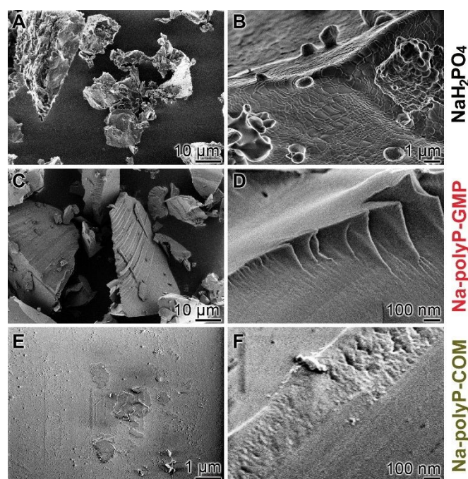
Fig. 2. Morphology of solid Na-polyP deposits and its NaH 2 PO 4 starting material; SEM. (A and B) Aspects of monomeric sodium phosphate. (C and D) Images of Na-polyP-GMP blocks. (E and F) The Na-polyP-COM samples show layers based on a granulated bottom (granulated particles).
