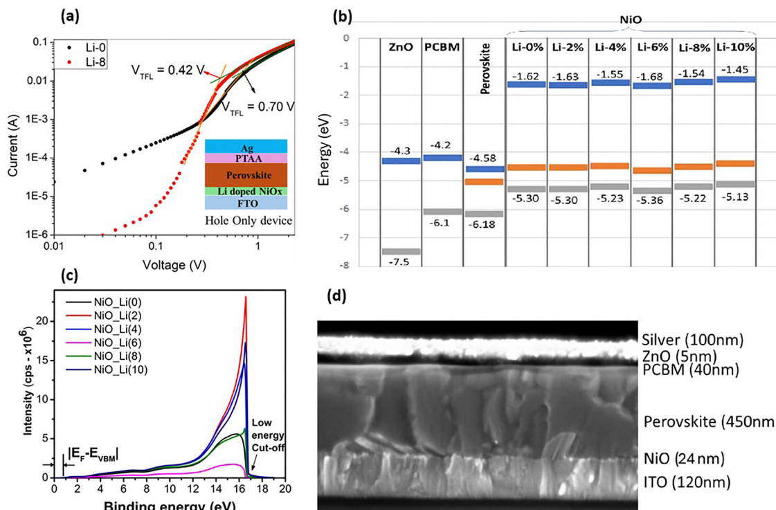
Fig. 3 (a) Dark JV curves and V TFL calculation for 0 and 8% Li-doped NiO x hole only devices (inset: device structure for hole only devices), (b) energy band alignment of perovskites with different Li-doped NiO x HTLs, (c) UPS characterization of different Li-doped NiO x HTLs, and (d) cross-sectional SEM image of the perovskite solar cell device.
