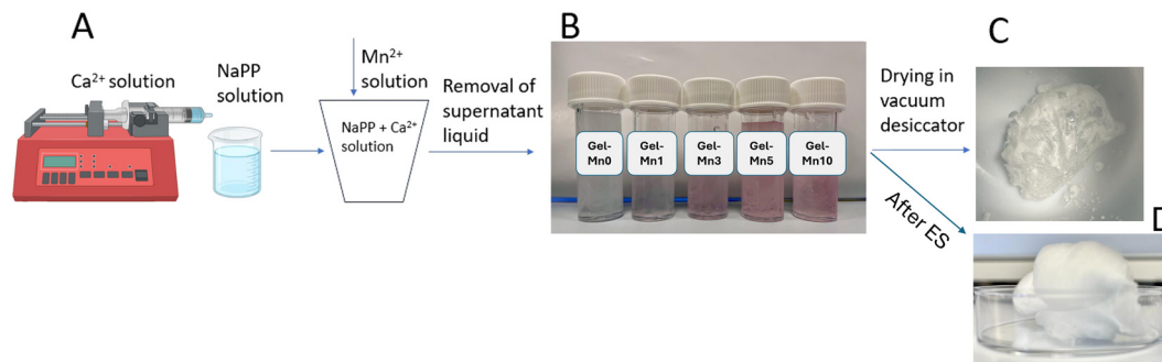
Fig. 1 (A) Schematic of the synthesis of PGs via coacervation; (B) images of all coacervate gels; (C) PGP-Mn0 in the system P 2 O 5 -CaO-Na 2 O obtained after drying of the coacervate Gel-Mn0 in a vacuum desiccator; (D) cotton-like bundle of PGF-Mn0 after ES of Gel-Mn0.
