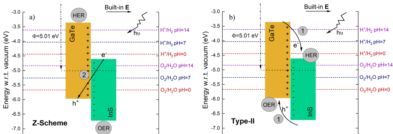
Fig. 9 The InS/GaTe band alignment and built-in electric field from GaTe to InS in the InS/GaTe heterostructure for the Z-scheme (a) and the type-II (b). Paths 1 and 2 illustrate the charge transfer mechanism of type-II and direct Z-scheme heterostructures, respectively. The dashed horizontal red, blue, and purple lines represent the reduction and oxidation potential of water with respect to vacuum at pH = 0, pH = 7, and pH = 14, respectively. The black dotted lines are the Fermi level of the InS/GaTe heterostructure.
