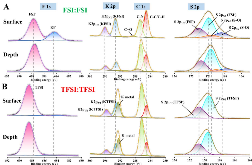
Fig. 6 XPS of the K metal surface and bulk (depth of 8 nm, Ar + etching speed of 0.8 nm min -1 ) after immersing for 28 days in (A) KFSI:Pyr 1201 FSI or (B) KTFSI:Pyr 1201 TFSI solutions (the grey open points represent the experimental data, and the solid lines represent the fitting results).
