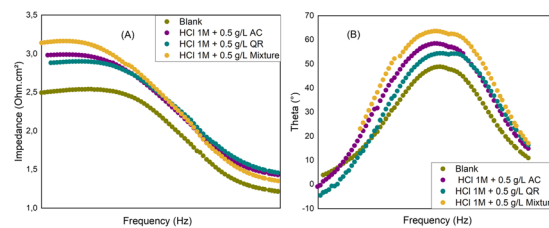
Fig. 6 (A) Bode impedance and (B) Bode theta spectra of the MS in the presence and the absence of 0.5 g L -1 of AC, QR and mixture in 1 M HCl at 293 K.
