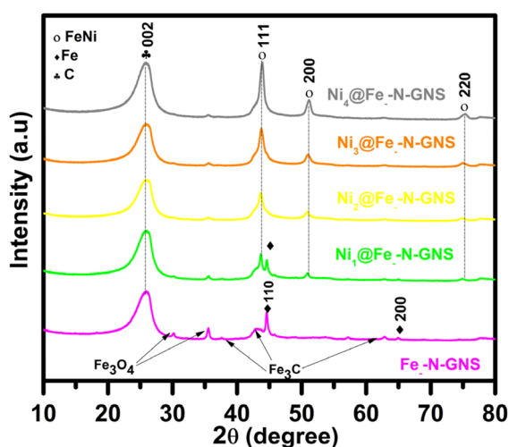
Fig. 1 XRD patterns of \text{Ni}_1@Fe\text{-N-GNS} , \text{Ni}_2@Fe\text{-N-GNS} , \text{Ni}_3@Fe\text{-N-GNS} , \text{Ni}_4@Fe\text{-N-GNS} , and Fe-N-GNS (synthesized without the nickel precursor).
