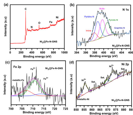
Fig. 2 XPS spectra of \text{Ni}_3@Fe\text{-N-GNS} : (a) survey spectrum, core-level XPS spectra in the (b) N 1s, (c) Fe 2p, and (d) Ni 2p regions.
