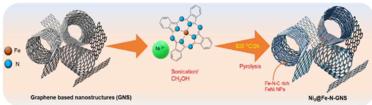
Scheme 1 A schematic representation of the \text{Ni}_3@Fe\text{-N-GNS} catalyst preparation process.
