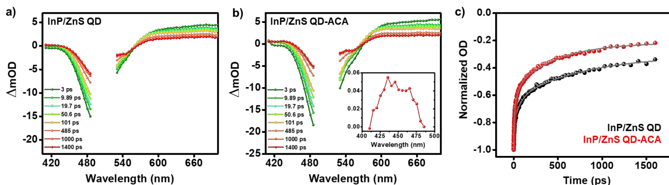
Fig. 2 fs-TA spectra at indicated time delays upon 500 nm excitation of a) InP/ZnS QDs and b) InP/ZnS QD-ACA. Inset of (b) shows the absorption feature of ^3ACA^* at ~430 nm obtained by subtracting the normalized spectra corresponding to 1400 ps and 3 ps time delays. c) Kinetics of the GSB bleach recovery of InP/ZnS QDs with and without ACA ligands.
