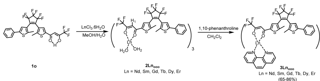
Scheme 1 Synthetic pathway yielding new complexes 3\text{Ln}_{\text{ooo}} ( \text{Ln} = \text{Nd, Sm, Gd, Tb, Dy, Er} ).
