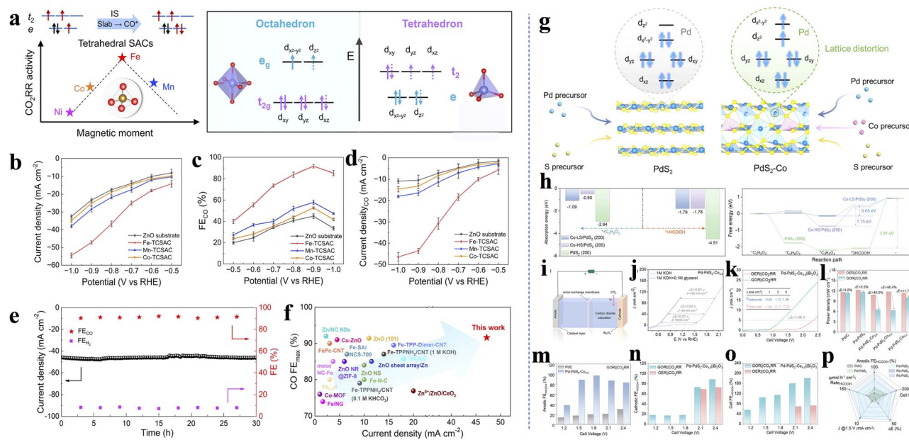
Fig. 14 (a) Electronic structures of TCSACs and schematic electron distribution. (b) Potential dependent performance of TCSACs: total current density. (c) CO. (d) Partial current density. (e) Time-dependent FE and current density of Fe-TCSAC at -0.9 \text{ V} vs. RHE for \text{CO}_2\text{RR} . (f) \text{FE}_{\text{CO}} and current density of Fe-TCSACs compared with those of other recently reported Zn/Fe-based catalysts. Reproduced with permission. 115 Copyright 2025 American Chemical Society. (g) Lattice distortion can induce different Pd d-orbital states of \text{PdS}_2 and \text{PdS}_2\text{-Co} models. (h) The adsorption energy of glycerol and formic acid on three models and free energy diagram of glycerol electrooxidation to formic acid pathway on three models. (i) Scheme of integrated electrolysis cell. (j) LSV curves of the integrated cell on \text{Pd-PdS}_2\text{-Co}_{4.0} . (k) The LSV curves of the integrated cell on \text{Pd-PdS}_2\text{-Co}_{4.0} . (l) The power density of the integrated cell at a current of 5 \text{ mA cm}^{-2} . (m) The anodic FE of \text{HCOOH} in GOR coupling with \text{CO}_2\text{RR} on \text{Pd-PdS}_2\text{-Co}_{4.0} and \text{Pd/C} . (n) The cathodic and (o) integrated cell FE of \text{HCOOH} on \text{Pd-PdS}_2\text{-Co}_{4.0} . (p) Overall performance comparison among various electrocatalysts. Reproduced with permission. 119 Copyright 2025 Wiley-VCH.
