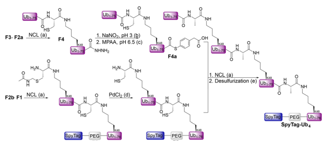
Fig. 4 Synthetic scheme for the synthesis of SpyTag-Ub 4 . All reactions were performed in 6 M Gnd-HCl, 200 mM NaPi. (a) 30 eq. TCEP, 50 eq. MPAA, pH 7, 37 °C; (b) 20 eq. NaNO 2 , pH 3, -15 °C; (c) 60 eq. MPAA, pH 6.5, rt; (d) 15 eq. PdCl 2 , 37 °C; (e) 250 mM TCEP, 120 eq./cysteine VA-044, 10% tBuSH, pH 7, 42 °C.
