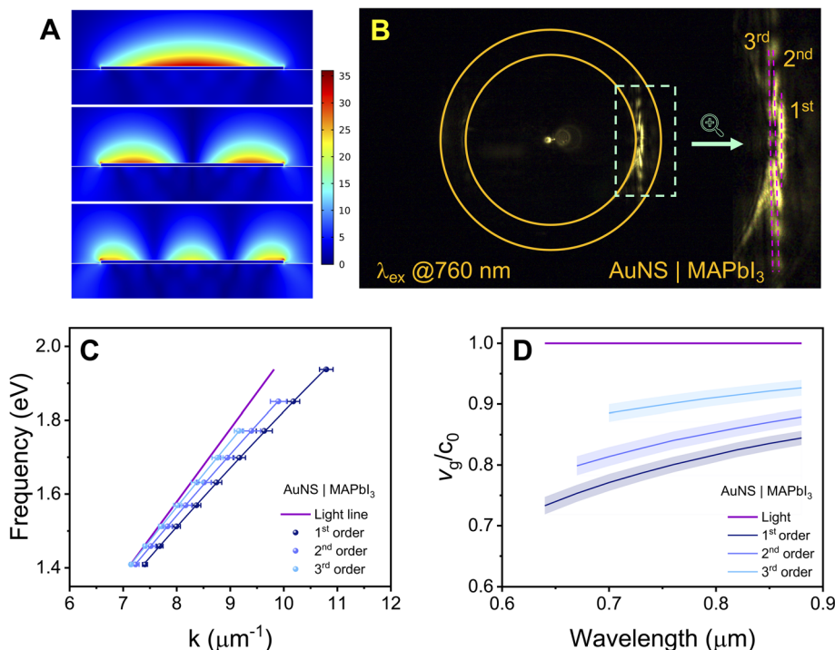
Fig. 2 (A) Plots of the normalized electric field from finite element simulations for the 1st, 2nd and 3rd order leaky modes of a 3 μm wide AuNS. In these plots air is on the top and glass is on the bottom. (B) Back focal plane image of a AuNS coated with a 14 nm MAPbI 3 layer at an excitation wavelength of 760 nm where multiple order leaky modes can be clearly seen. (C) Dispersion curves for the different order leaky modes in the 14 nm AuNS/MAPbI 3 heterostructures. (D) Group velocity profiles for the different leaky SPP modes in the 14 nm AuNS/MAPbI 3 heterostructures, normalized to the speed of light in vacuum. Error bars correspond to 95% confidence limits.
