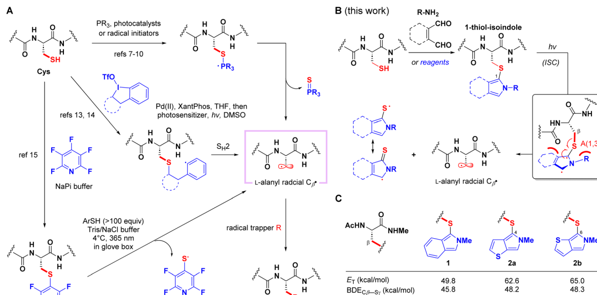
Fig. 1 Previous methods for radical desulfurative modifications of cysteine and the approach proposed in this study. (A) Phosphine-assisted desulfuration via phosphoranil radicals, S H2 strategy, and thiol activation through photoinduced electron transfer to fluoropyridines. (B) The postulated photo-induced C β -S bond homolysis based on the isoindole chromophore. (C) DFT calculations of three different chromophores; energy obtained at the (U)ωB97X-D/def2 TZVP/SMD(H 2 O)//(U)ωB97X-D/def2-SVP/SMD(H 2 O) level.
