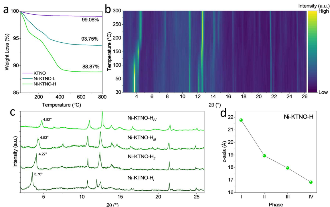
Fig. 2 (a) TGA of KTNO, Ni-KTNO-L and Ni-KTNO-H up to 800 °C. (b) in situ variable temperature XRD between 30 °C and 300 °C. (c) individual patterns at 30 °C (i), 150 °C (ii), 300 °C (iii) and 400 °C (iv). (d) The change in the c -axis of phases I–IV.
