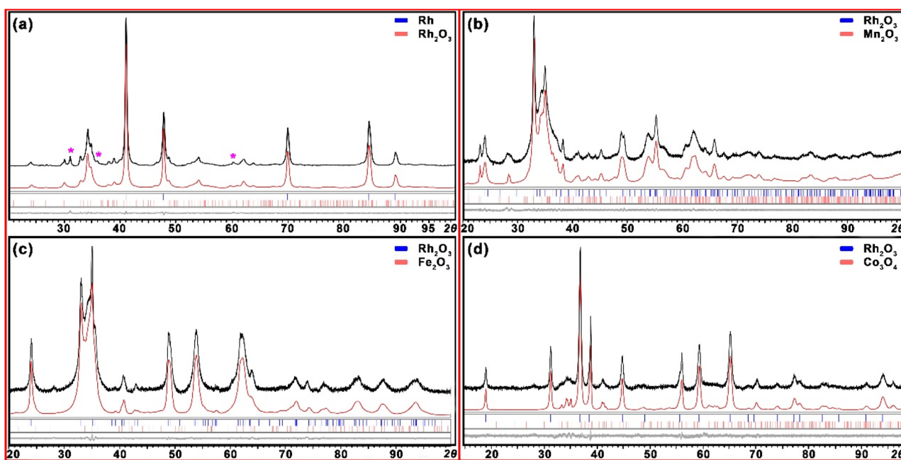
Fig. 3 Powder X-ray diffraction patterns of the residues obtained by thermal decomposition of [Rh(acac) 3 ] (a) and molecular precursors 1–3 (b–d, respectively) with the Le-Bail fit. Black and red curves represent experimental and calculated patterns, respectively. Gray is the difference curve with theoretical peak positions shown as blue and red bars at the bottom. Impurity peaks are marked with asterisk.
