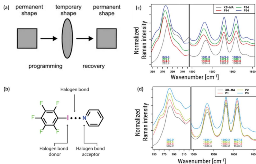
Fig. 9 (a) Operation steps of the shape memory polymers (b) vibrational modes of C–X bonds in halogen bonded polymer with focus on the I...N interactions. (c) and (d) Raman spectrum of 3D-printable shape memory polymers based on halogen bonding to confirm molecular structure of the polymer. All figures are reproduced with permission.
