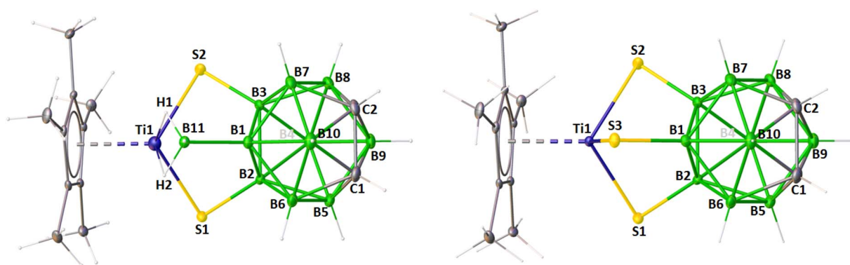
Fig. 5 Molecular structure and labelling diagram of 3 (left) and 4a (right). Selected bond lengths ( \text{\AA} ) and bond angles ( ^\circ ): 3 : \text{Ti}1\text{-S}1 2.3321(9) , \text{Ti}1\text{-S}2 2.3214(9) , \text{Ti}1\cdots\text{B}11 2.259(4) , \text{Ti}1\text{-H}1 2.00(3) , \text{Ti}\text{-H}2 1.93(3) , \text{B}11\text{-H}1 0.90(3) , \text{B}11\text{-H}2 1.03(4) , \text{B}1\text{-B}11 1.750(5) , \text{B}2\text{-S}1 1.851(4) , \text{C}1\text{-C}2 1.626(6) , \text{Ti}1\text{-S}1\text{-B}2 81.17(11) , \text{B}2\text{-B}1\text{-B}11 121.9(3) . 4a : \text{Ti}1\text{-S}1 2.3095(12) , \text{Ti}1\text{-S}3 2.3231(12) , \text{B}1\text{-S}3 1.849(5) , \text{B}1\text{-B}2 1.829(5) , \text{C}1\text{-C}2 1.635(7) , \text{C}1\text{-B}10 1.713(7) , \text{Ti}1\text{-S}1\text{-B}2 80.72(14) .
