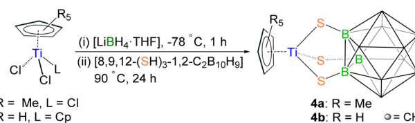
Scheme 3 Synthesis of 8,9,12-trithiol-o-carborane protected Ti-thiolate complexes 4a and 4b .
