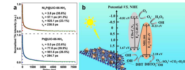
Fig. 11 (a) The transient absorption kinetics of Ni 2 P@UiO-66-NH 2 and Pt@UiO-66-NH 2 . 98 Copyright 2020, John Wiley and Sons. (b) Photocatalytic mechanism of the Z-scheme heterojunction in MIL101/CDs-C 3 N 4 for ENR degradation. 106 Copyright 2024, John Wiley and Sons.
