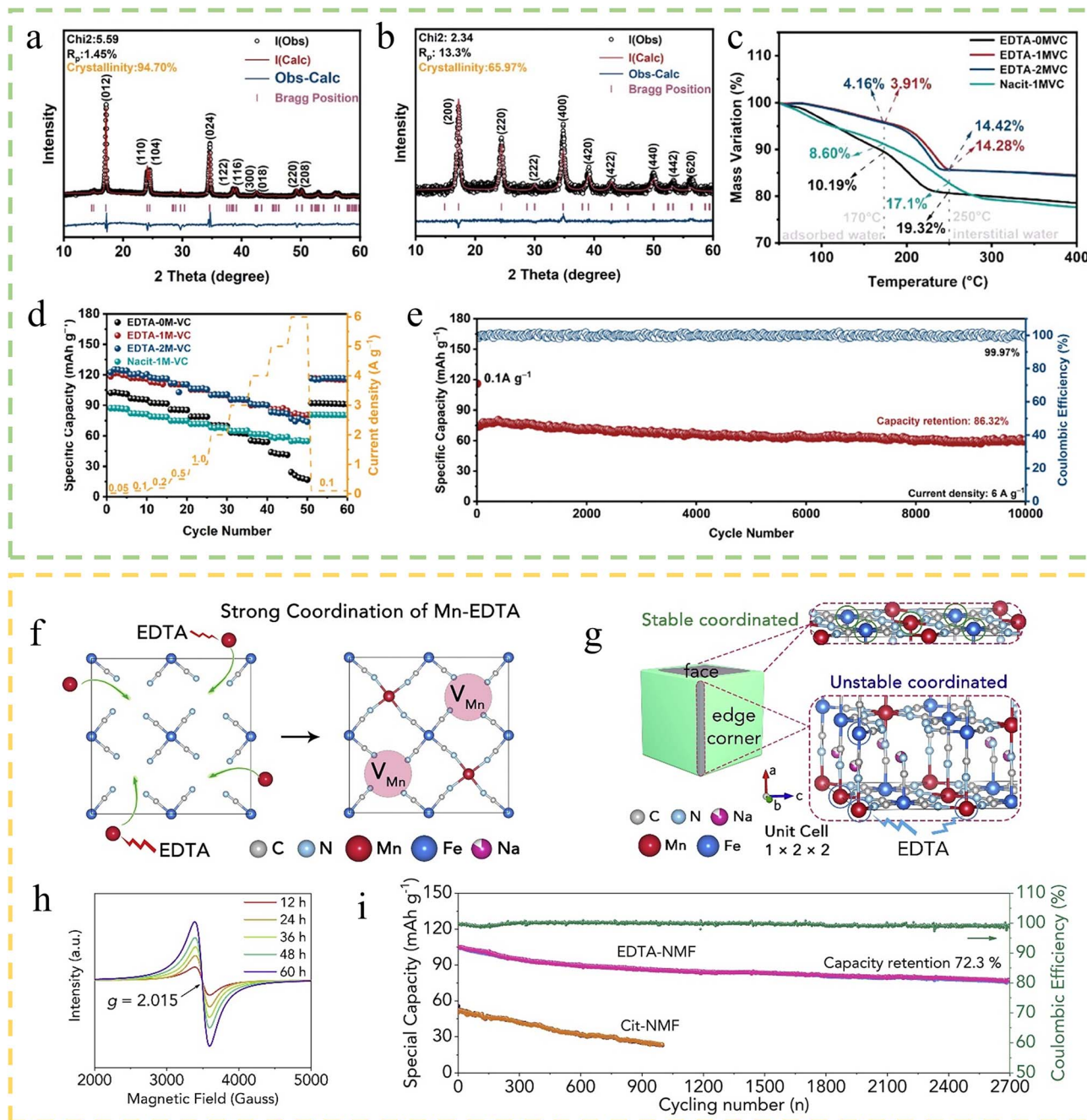
Fig. 8 (a) Rietveld refinement XRD pattern of EDTA-1MVC (b) Nacit-1MVC. (c) TGA comparison curve in \text{N}_2 . (d) Rate performance of all the cathodes. (e) Long-term cycling performance of EDTA-1MVC at 6 \text{A g}^{-1} after 10 cycles at 0.1 \text{A g}^{-1} . 122 Copyright 2024, Wiley-VCH. (f) The formation mechanism of Mn vacancies in NMF. (g) Etching mechanism of NMF with \text{Na}_2\text{EDTA} . (h) ESR spectra of EDTA-NMF obtained at different reaction times. (i) Cycling performances of two NMFs at 500 \text{mA g}^{-1} and the coulombic efficiency of hexapod EDTA-NMF. 123 Copyright 2020, Elsevier.
