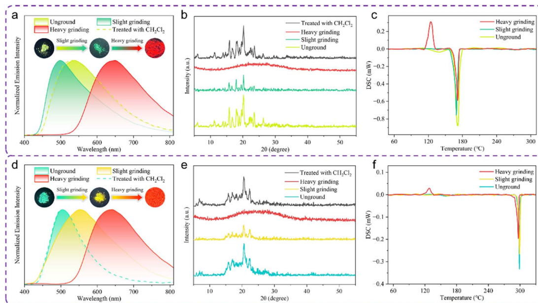
Fig. 2 Normalized PL spectra and PL photographs under 365 nm UV light of the as-synthesized, slightly ground, and heavily ground solid states of Sym- m -OMe (a), Sym- p -OMe (d). PXRD patterns of Sym- m -OMe (b) and Sym- p -OMe (e) in various solid states. DSC curves of Sym- m -OMe (c) and Sym- p -OMe (f) in various solid states. The scan rate is 5 °C min -1 under N 2 .
