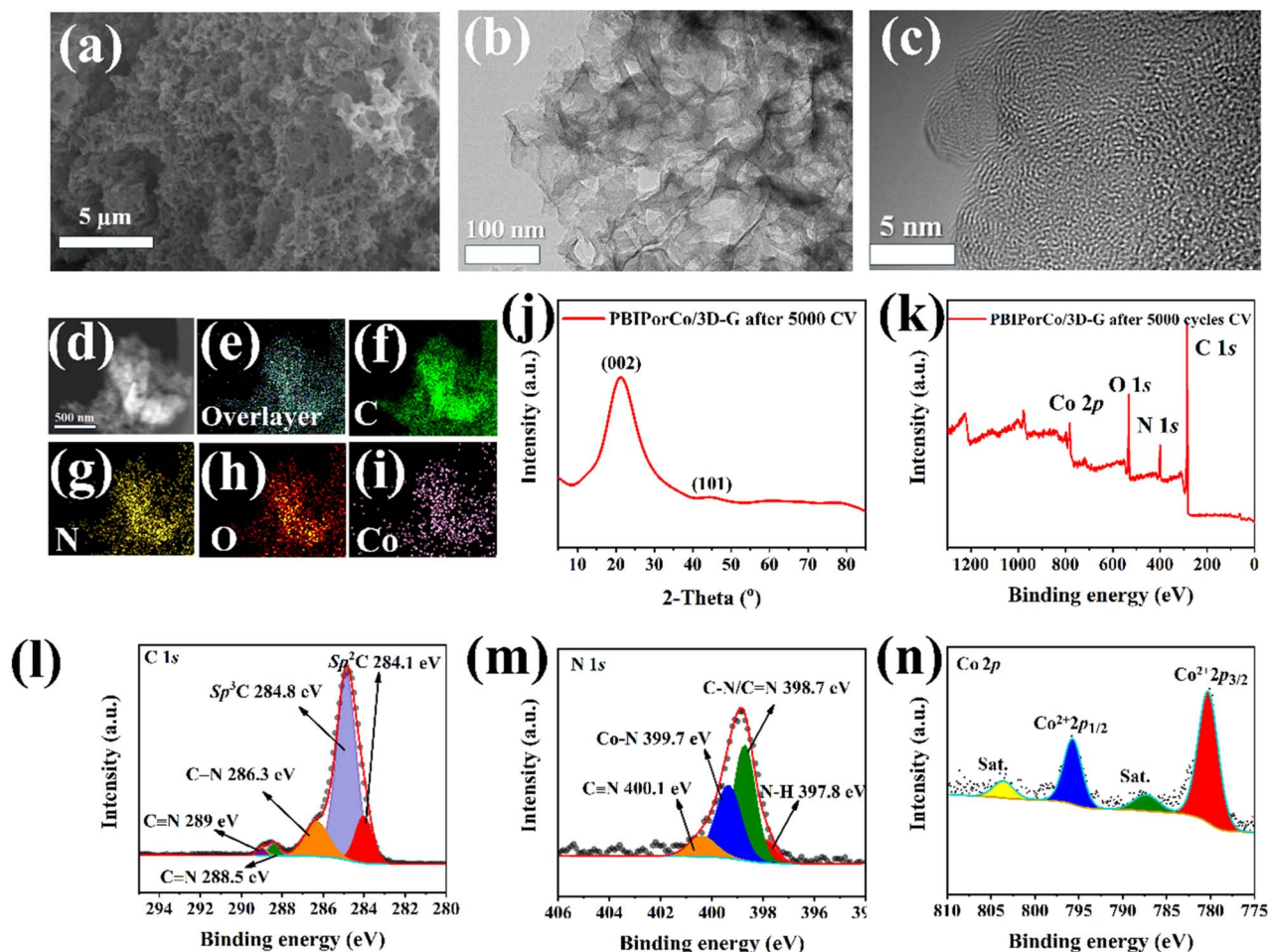
Fig. 5 Composition, morphology, structure and valence state characterization after durability testing. (a) SEM of PBIPorCo/3D-G-5000; (b) and (c) TEM and HR-TEM of PBIPorCo/3D-G-5000; (d) HAADF-STEM; (e–i) mapping of overlayer, C, N, O, and Co; (j) XRD of PBIPorCo/3D-G-5000; (k) XPS full spectra; (l–n) high-resolution XPS spectra of PBIPorCo/3D-G-5000: C 1s, N 1s, and Co 2p.
