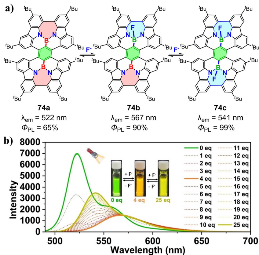
Fig. 25 (a) Double-fluoride titration of double-boron doped helicene 74a . (b) Titration experiments of 74a in acetone ( 1.0 \times 10^{-5} \text{ M} ) solution with TBAF, measured using fluorescence spectra ( \lambda_{ex} = 470 \text{ nm} ). Inset: photographs showing fluorescence of 74a with 0 equiv., 4.00 equiv. and 25 equiv. of TBAF in acetone. Copyright 2023, John Wiley & Sons.
