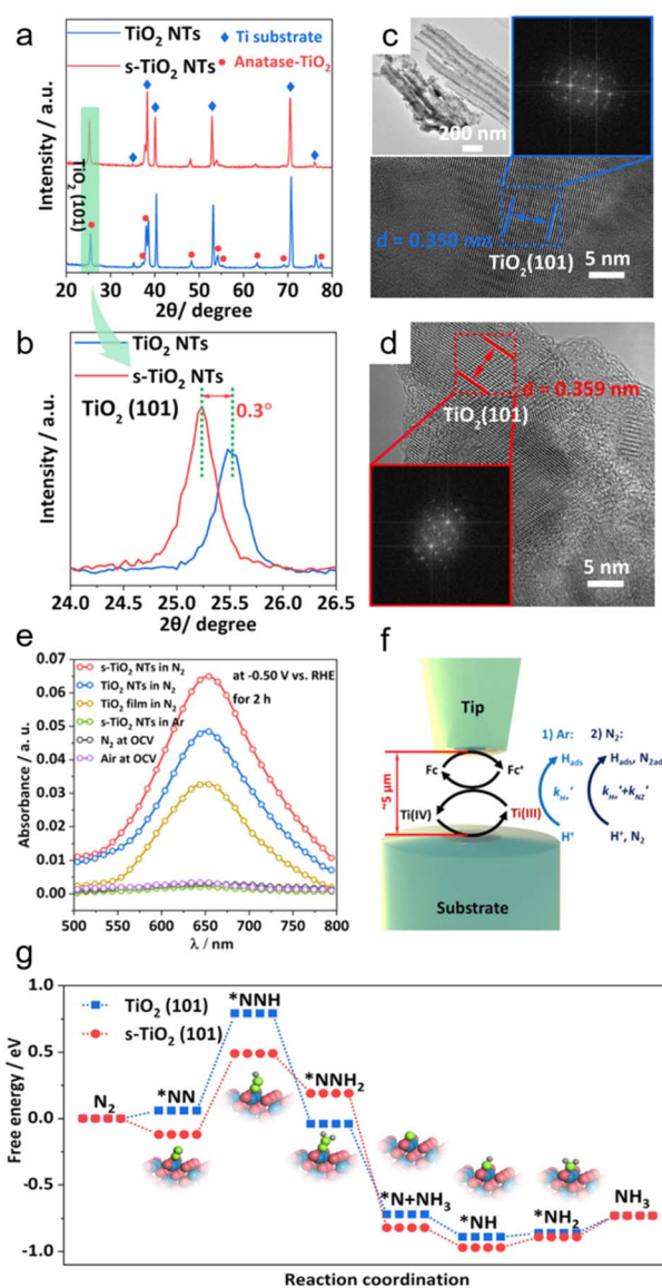
Fig. 2 (a and b) XRD patterns of TiO 2 NTs and s-TiO 2 NTs. (c and d) TEM images and the corresponding fast Fourier transform (FFT) patterns (the inset) of TiO 2 NTs (c) and s-TiO 2 NTs (d). (e) UV/vis absorption spectra of the electrolyte with an indophenol indicator after 2 h of electrolysis at –0.5 V. (f) Illustration of SI-SECM for determining the reaction rate constants of H + and N 2 adsorption on the Ti 3+ site in TiO 2 NTs and s-TiO 2 NTs. (g) DFT-calculated pathways of the NRR through the distal mechanisms on pristine and strained TiO 2 (101). Reproduced with permission from ref. 92, John Wiley and Sons, 2020.
