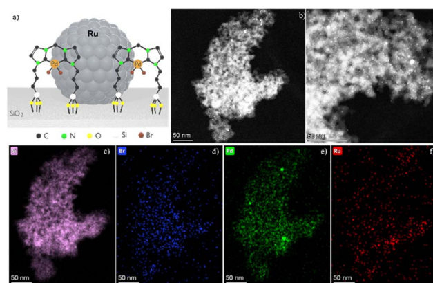
Fig. 5 Schematic depiction (a), and electron microscopy (b)–(f) of \text{Ru@SiO}_2 - [\text{Pd-NHC}] . (b) STEM-HAADF, and (c)–(f) EDX elemental mapping of (c) Si– K\alpha ; (d) Br– K\alpha ; (e) Pd– L\alpha ; (f) Ru– K\alpha .
