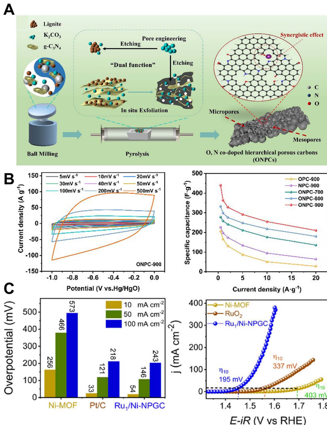
Fig. 5 (A) Schematic of synergistically fabricated ONPC materials. 33 (B) CV plots of ONPC-900 measured at various scans (5–500 mV s -1 ) and SC comparison of ONPC materials measured at different current densities. 33 Reuse permission from Liu et al. (2025) 33 by OAE Publishing Inc., under a Creative Commons Attribution 4.0 International License ( https://creativecommons.org/licenses/by/4.0/ ). (C) HER performance of Ru 1 /Ni-NPGC catalysts and iR -corrected OER polarization curves (scan rate 1 mV s -1 ). 13 Reuse permission from Mishra et al. (2025) 13 by The Royal Society of Chemistry.
